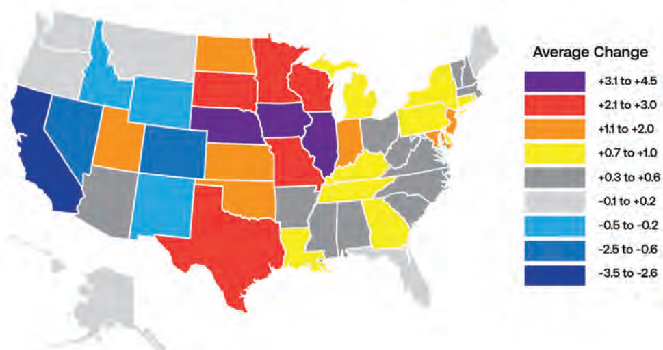
Average Change in Ozone Weighted Average by State 2020-2022 to 2021-2023
